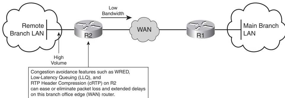
Figure 2-2 Solutions for Packet Loss and Extended Delay
