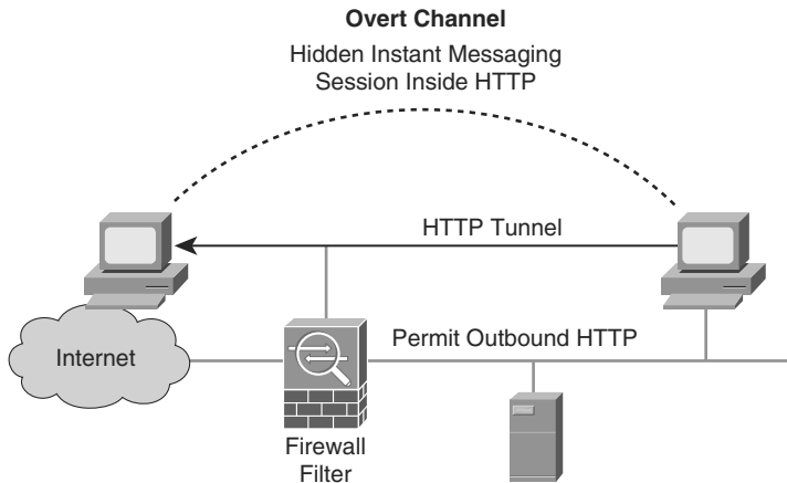
Figure 1-9 Overt Channel
