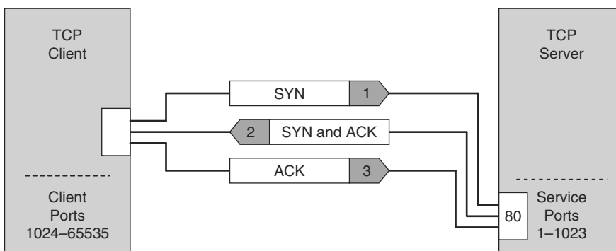
Figure 1-4 TCP Three-Way Handshake
