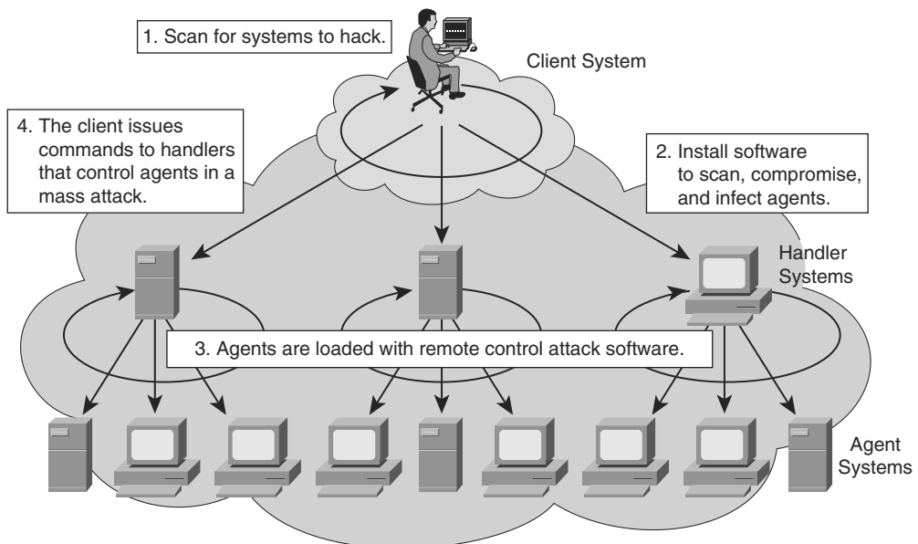
Figure 1-11 DDoS Attack
