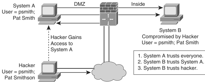
Figure 1-6 Trust Exploitation
