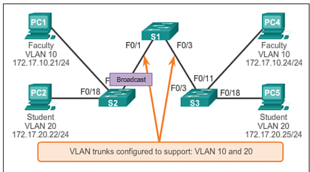
Figure 3-6 Broadcasts with VLAN Segmentation
