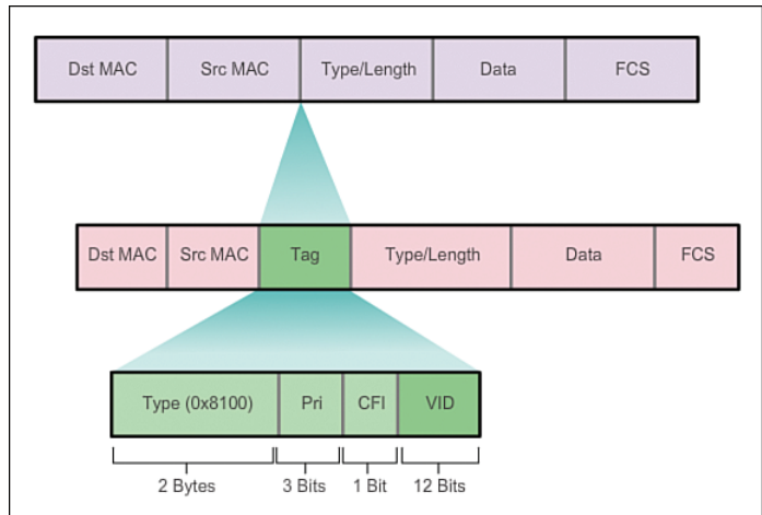
Figure 3-7 802.1Q VLAN Tag
