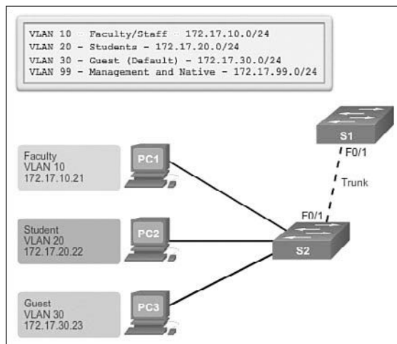
Figure 3-19 Sample VLAN Design
