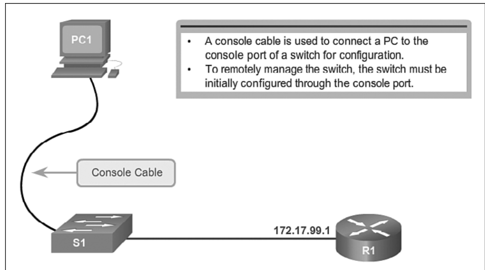
Figure 2-4 Preparing for Remote Switch Management
