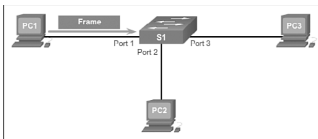
Figure 1-13 Building a MAC Address Table: PC1 Sends Frame to Port 1
