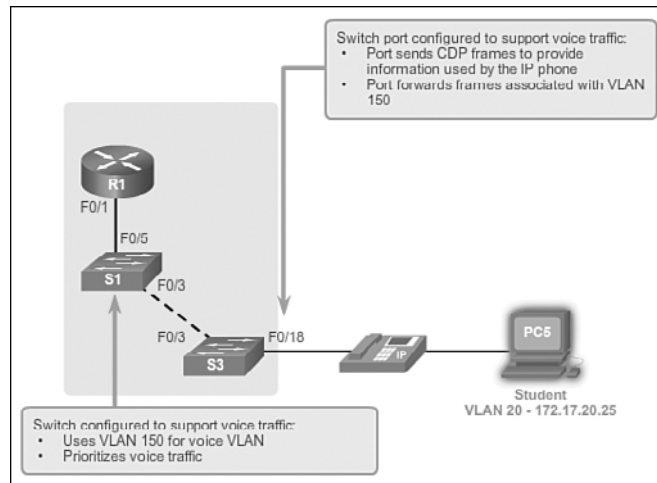
Figure 3-5 Voice VLAN
