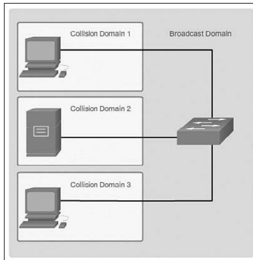
Figure 1-21 Collision Domains
