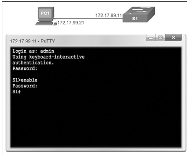
Figure 2-14 Remote Management SSH Connection
