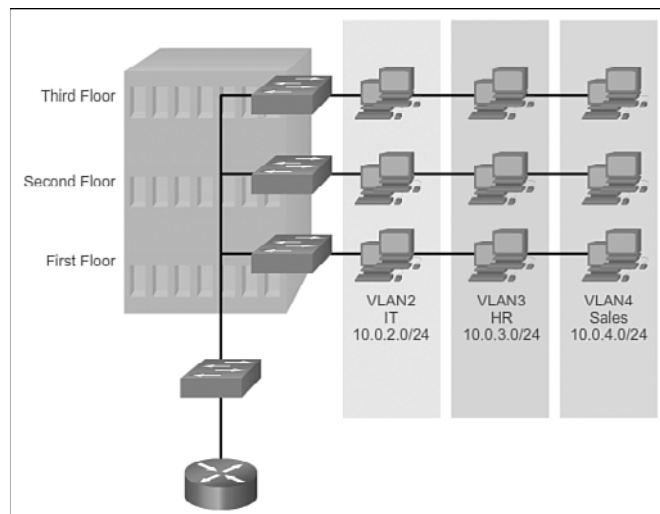
Figure 3-1 VLAN Groups
