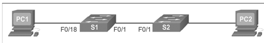
Figure 2-9 Configure Auto-MDIX
