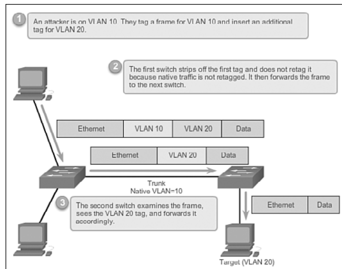
Figure 3-29 Double-Tagging Attack
