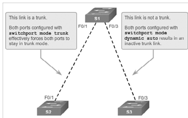
Figure 3-21 DTP Interaction Results
