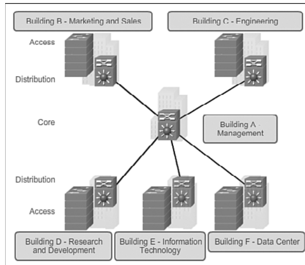
Figure 1-6 Three-Tier Campus Network Design
