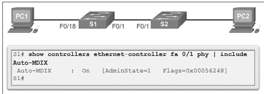
Figure 2-10 Verify Auto-MDIX
