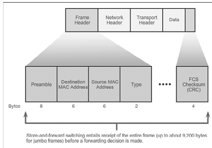
Figure 1-19 Store-and-Forward Switching
