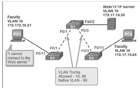
Figure 3-22 IP Issue Within a VLAN
