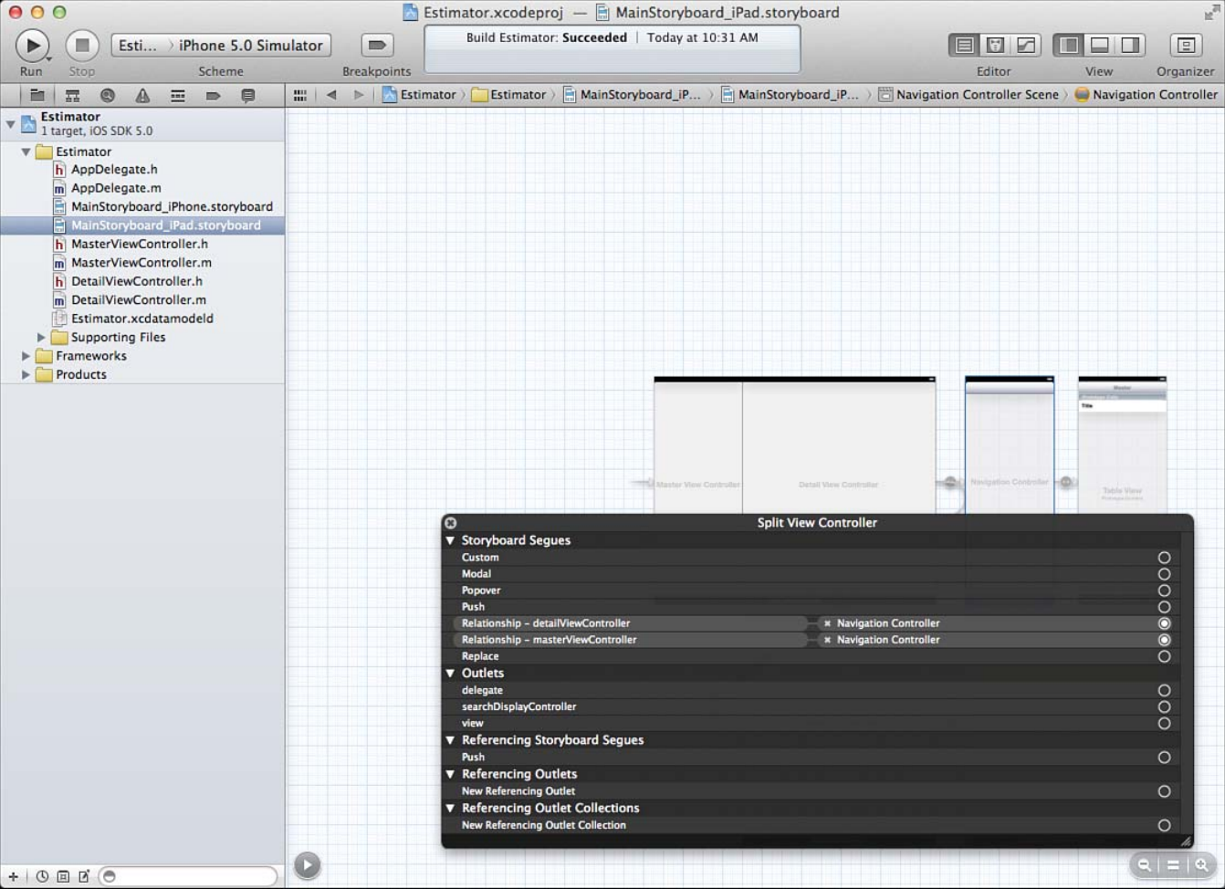
Figure 14.11 Review segues and outlets for a split view controller.
