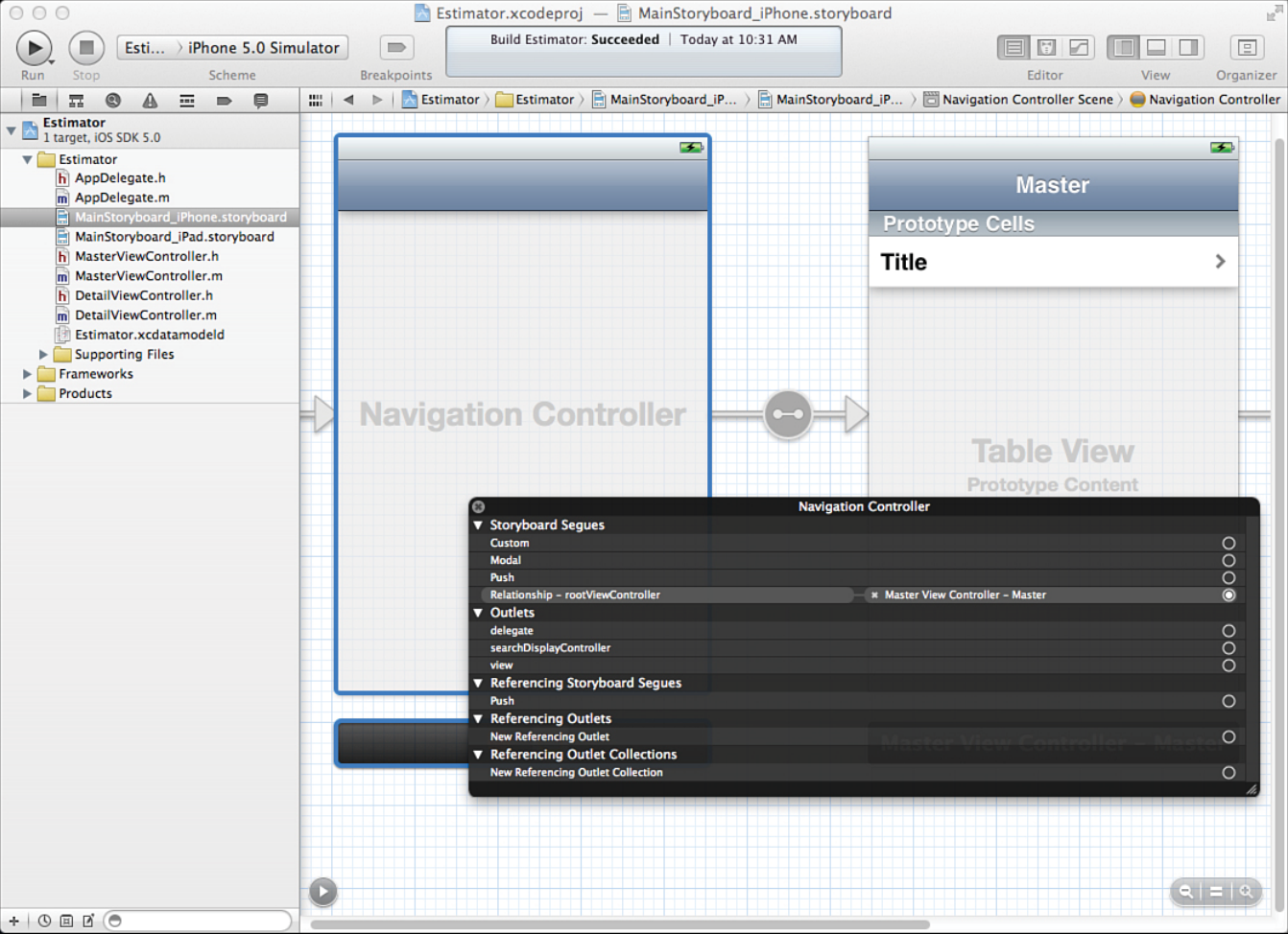
Figure 14.10 Review segues and outlets for a navigation controller.
