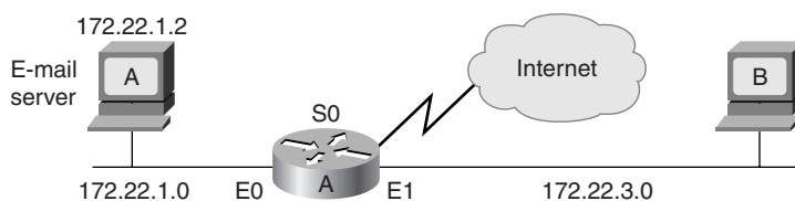
Figure A-15 Network Used for Extended IP Access List Example
