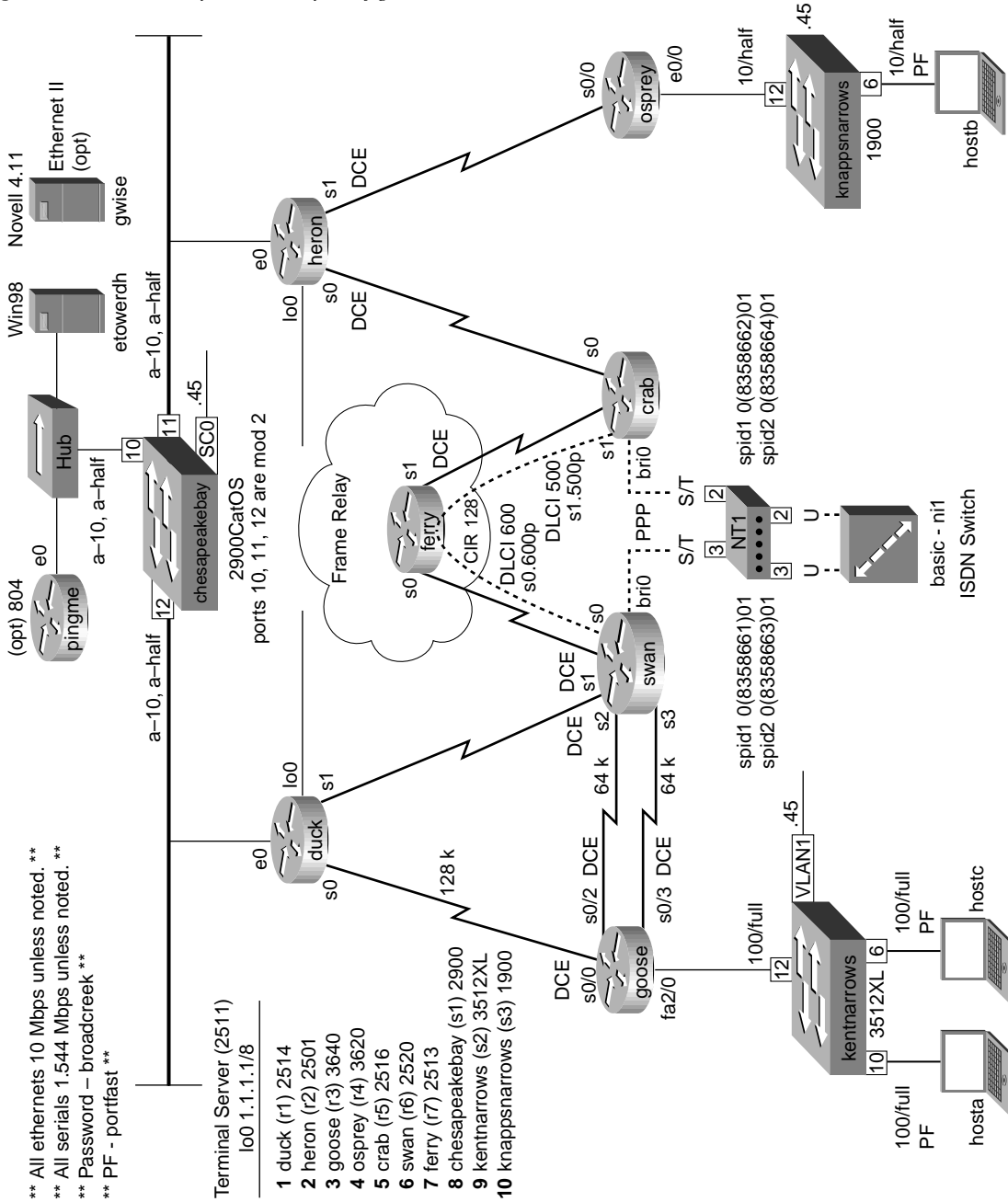
Figure 10-2 Lower-Layer Discovery/Configuration
