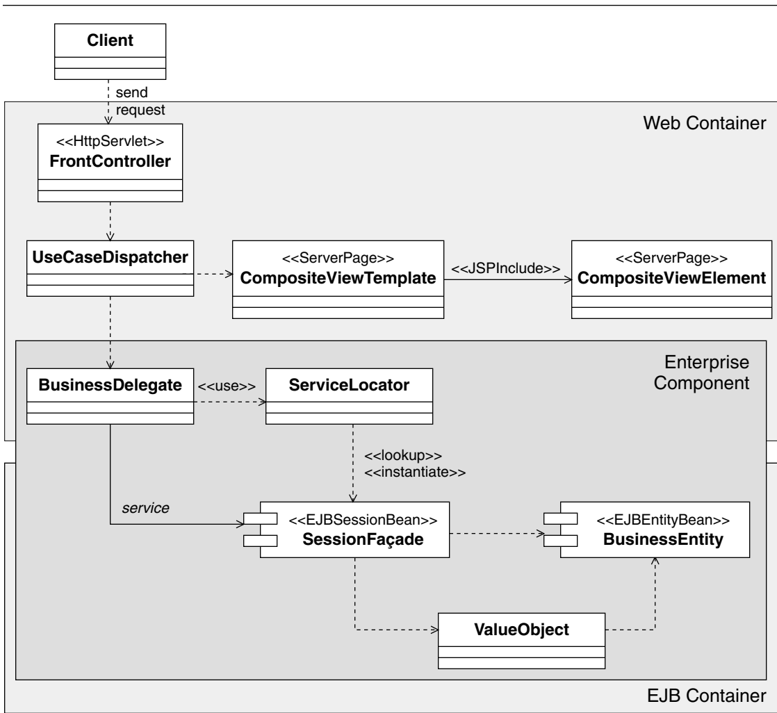
Figure 8.7 An Internal Perspective of an Enterprise Component and Allocation of Its Design Elements to Containers
