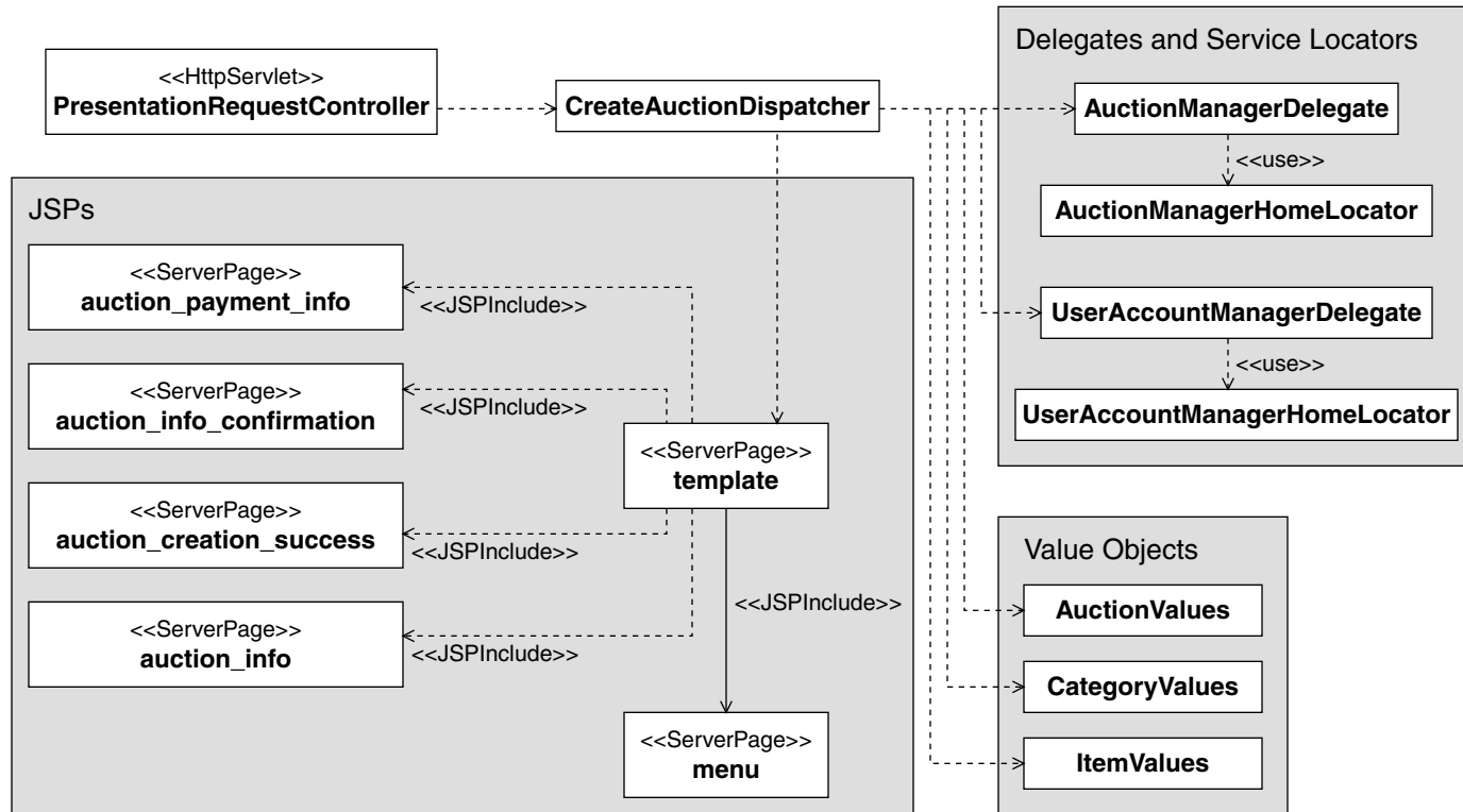
Figure 8.20 Participants in the Create Auction Use Case
