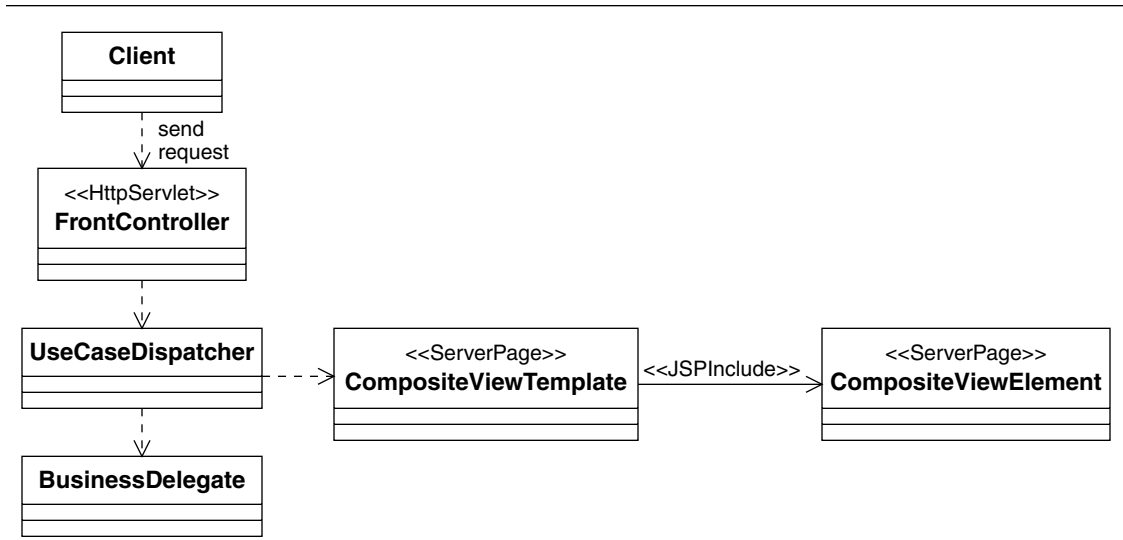
Figure 8.5 The Implementation Strategy for the Presentation Layer
