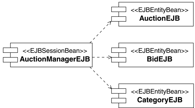
Figure 8.16 Auction Manager EJBs
