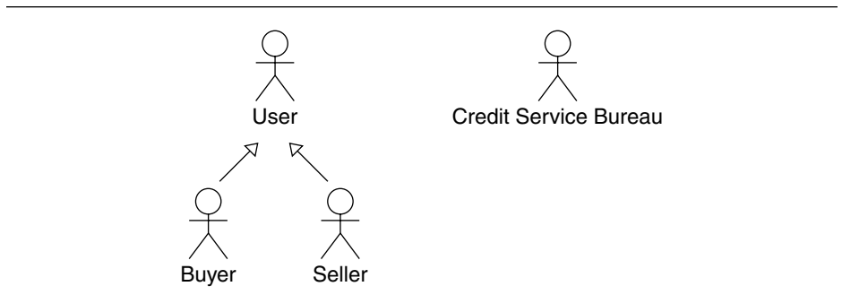
Figure 6.4 Online Auction Application Actors
