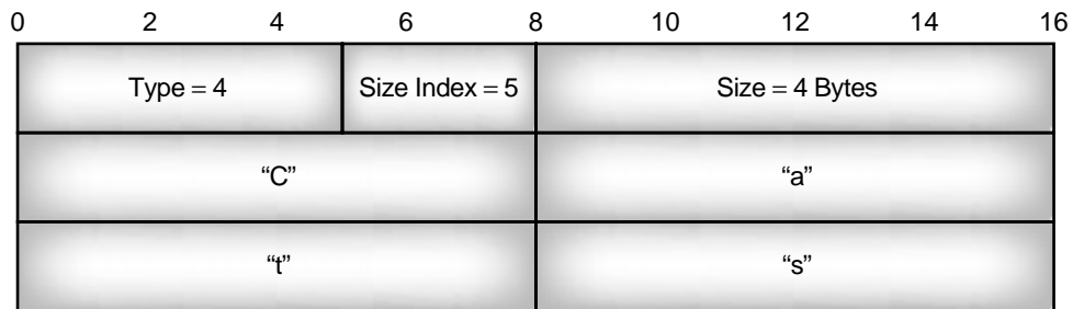
Figure 11-4 Data element containing a text string.
