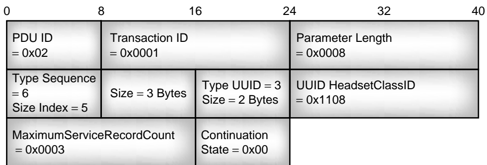
Figure 11-12 Structure of an SDP_ServiceSearchRequest.
