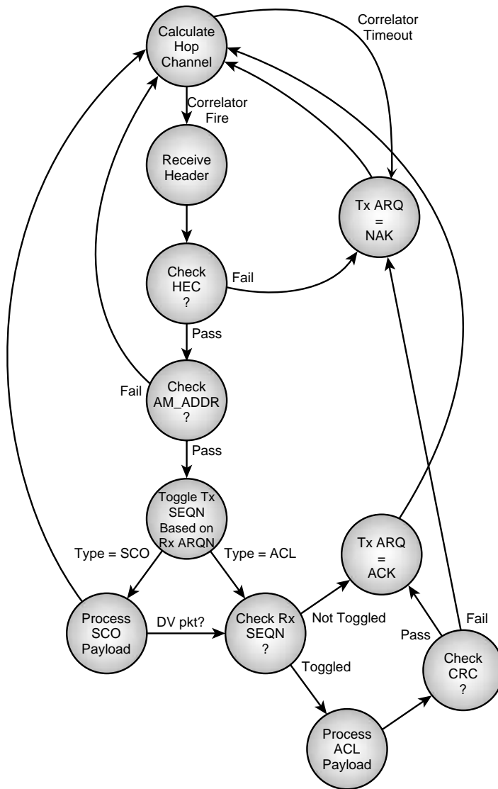
Figure 5-17 LC receive state machine.
