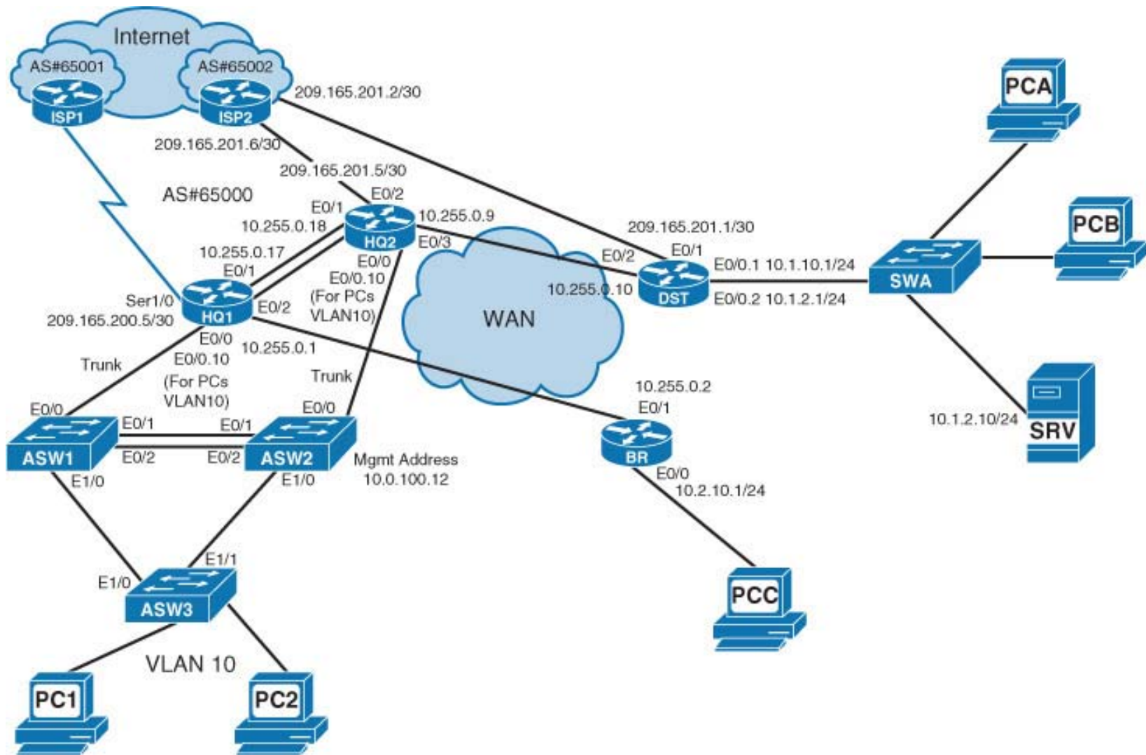
Figure 10-1 RADULKO Transport's Network Diagram
