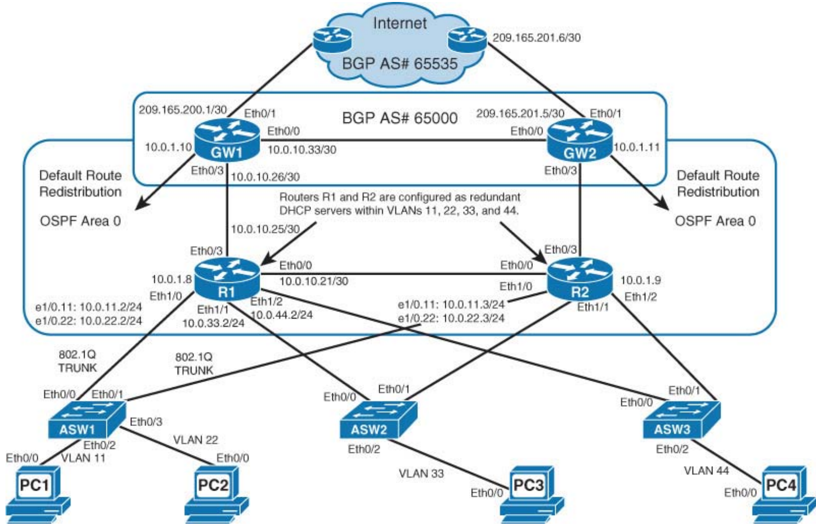
Figure 7-2 TINC Garbage Disposal Network Diagram
