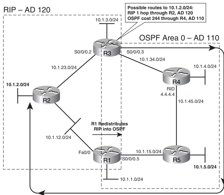
Figure 11-4 OSPF and RIP Redistribution
