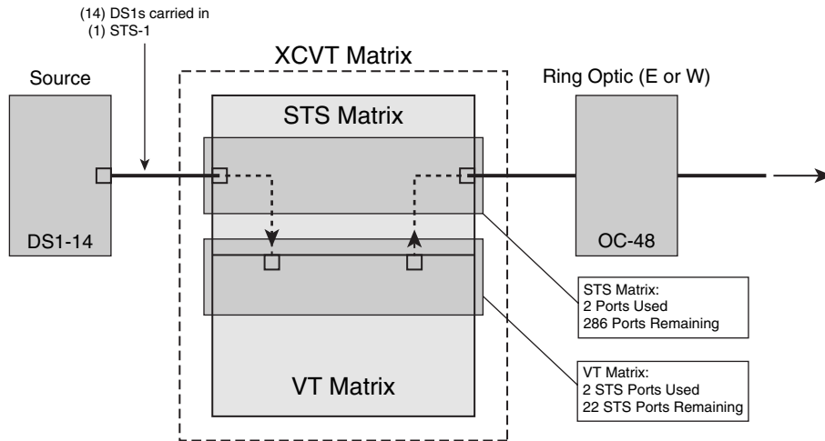
Figure 6-4 VT Matrix Use for a DS1 Circuit in a BLSR Termination Node
