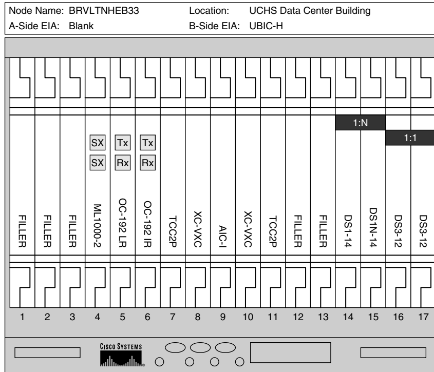
Figure 6-22 UCHS Data Center Node—Shelf Diagram
