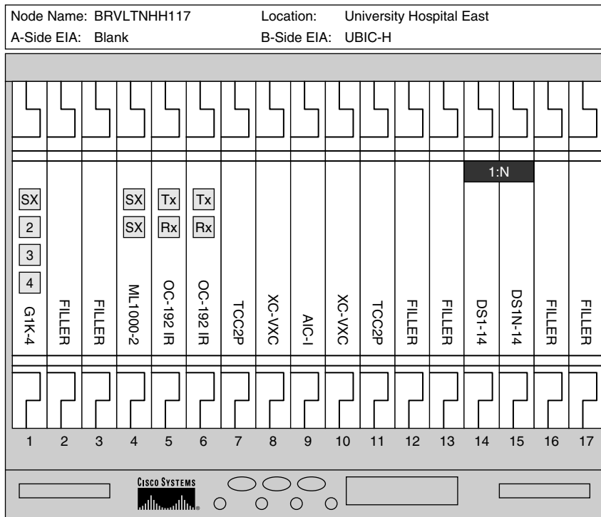
Figure 6-19 University Hospital—East Node—Shelf Diagram
