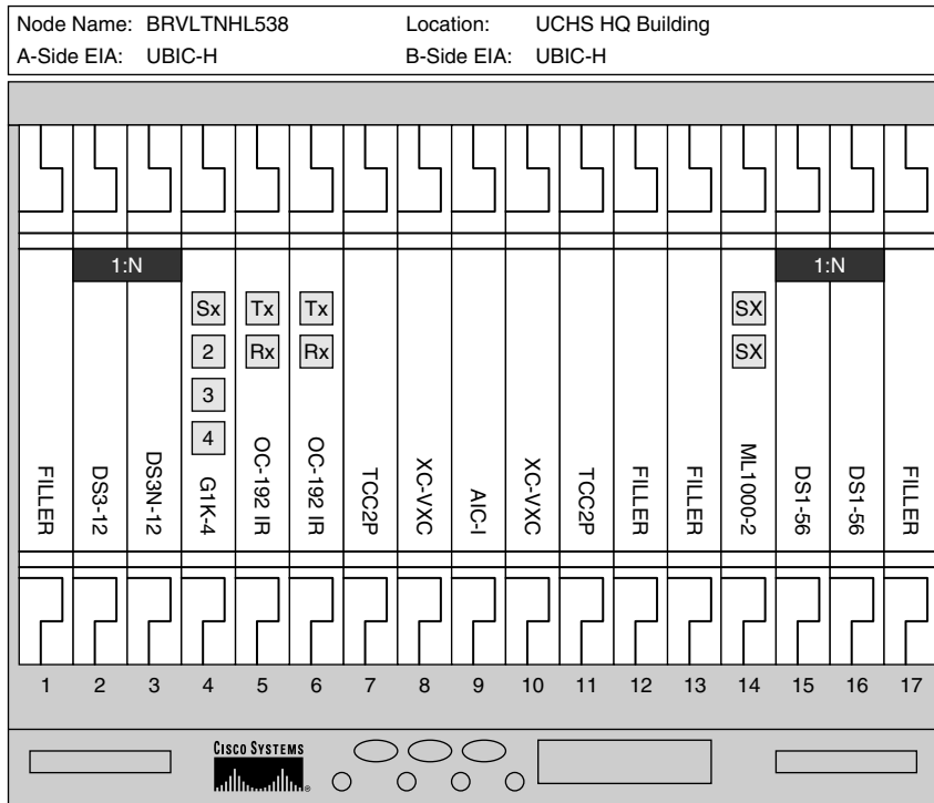
Figure 6-16 UCHS Headquarters Node—Shelf Diagram
