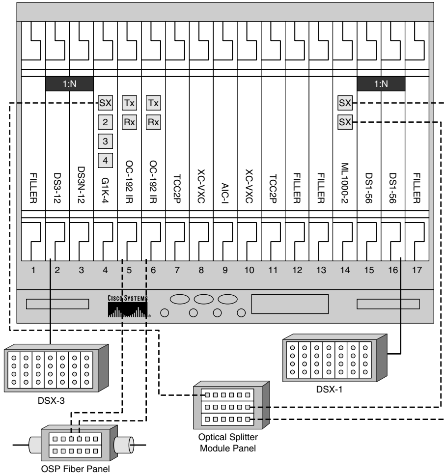
Figure 6-24 Cabling Termination Diagram, UCHS Headquarters Node
