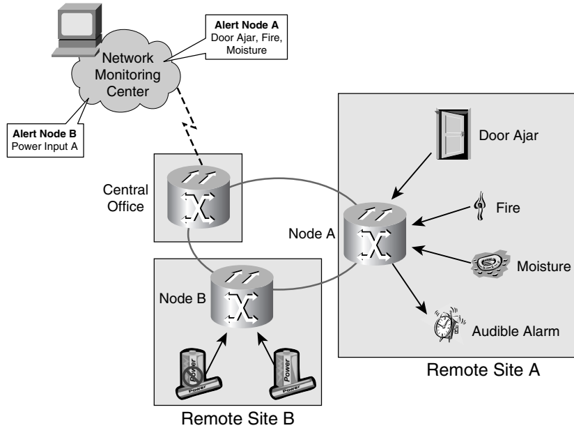
Figure 6-7 Environmental Alarms Reported Using AIC-I Card Interfaces
