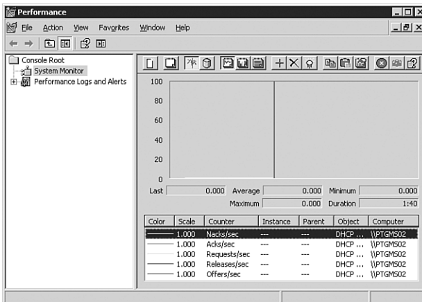
FIGURE 2.43 You can monitor DHCP server statistics in real time.
