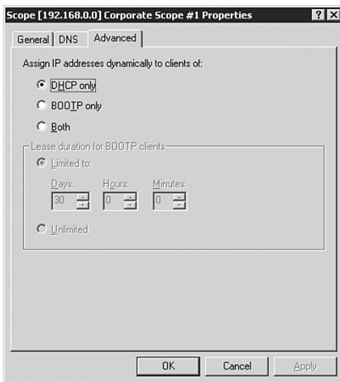
FIGURE 2.12 You can configure the scope to service BOOTP clients on the Advanced tab of the Scope Properties dialog box.
