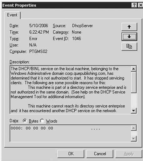
FIGURE 2.45 An unauthorized DHCP server cannot start the DHCP service.
