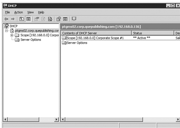
FIGURE 2.20 When a DHCP server is authorized, DHCP server scope information shows up in the right pane of the DHCP console window.
