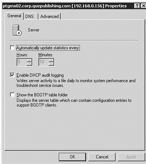
FIGURE 2.33 DHCP audit logging is enabled from the General tab of the DHCP server Properties dialog box.
