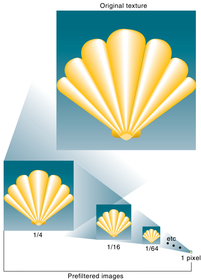
Figure 9-6 Mipmaps
