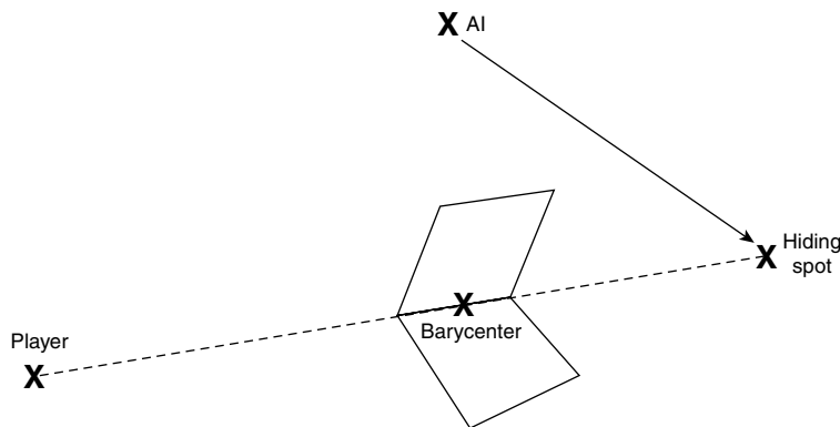
Figure 7.6 Geometry of playing hide-and-seek with the player.
