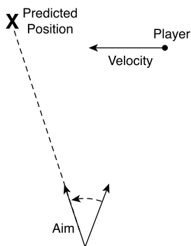
Figure 7.7 Predictive shooter.
